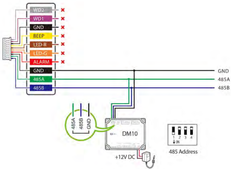
Figure 1-4 DM10 Wiring
