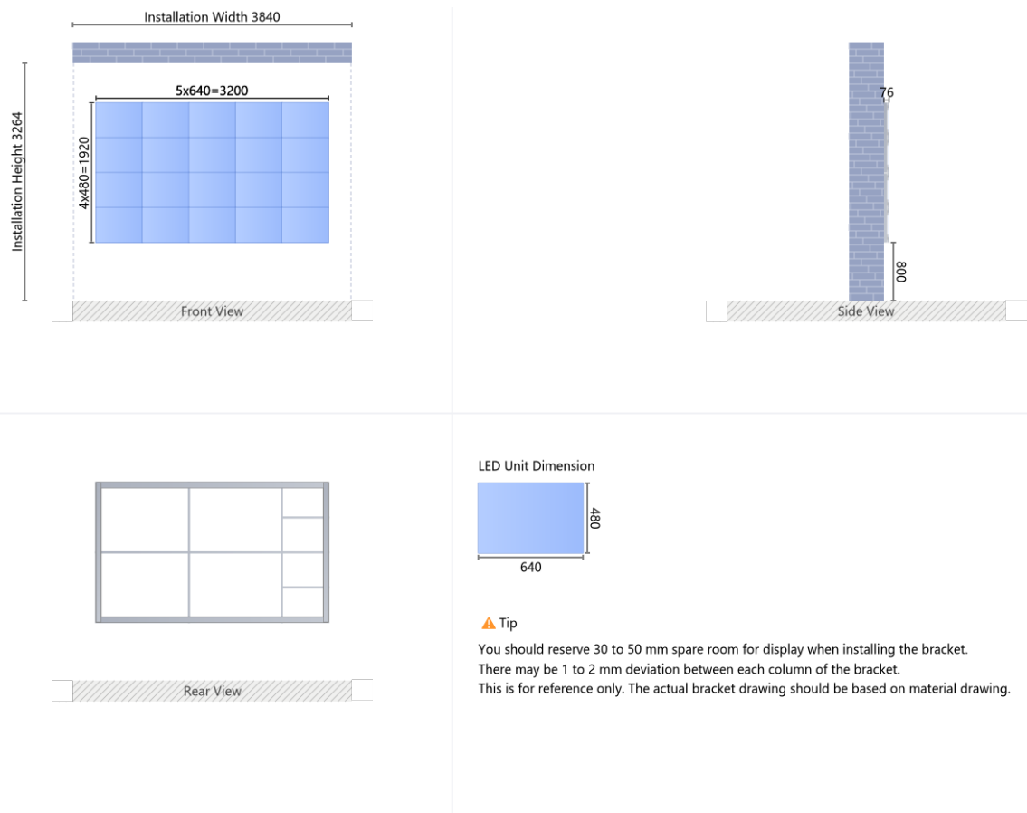
Figure 2.1.1 Bracket Installation
