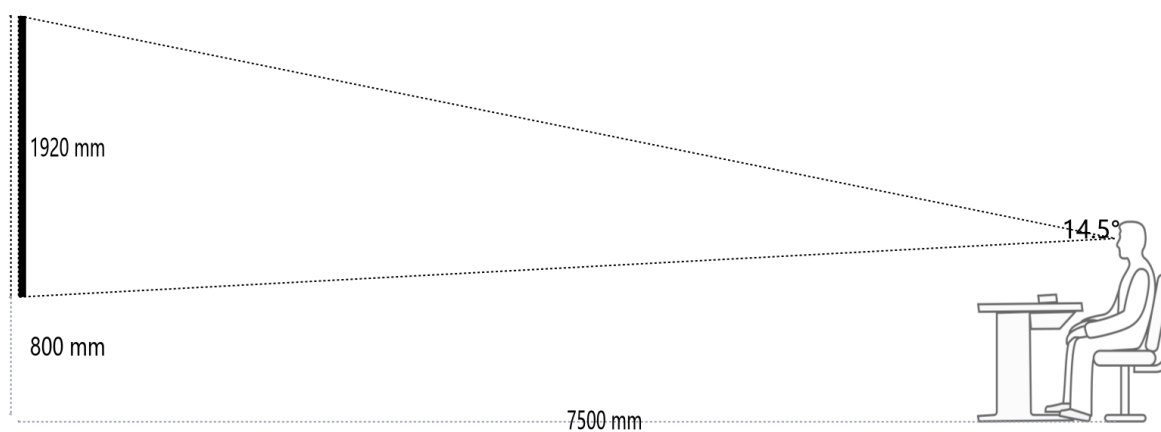
Figure 1.2.1 Side View
