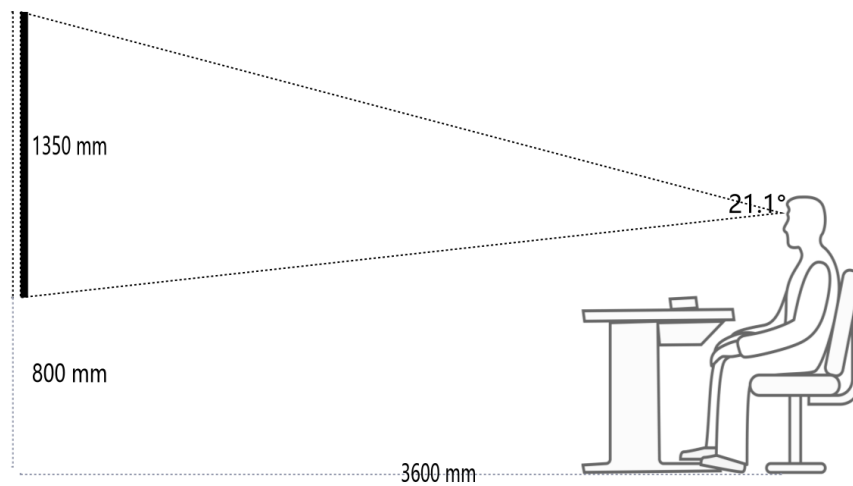
Figure 1.2.2 Vertical View
