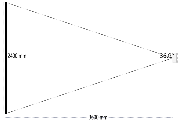
Figure 1.2.1 Side View
