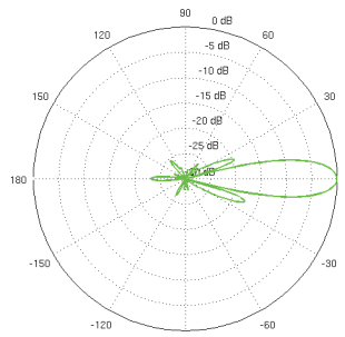
Horizontal Azimuth
