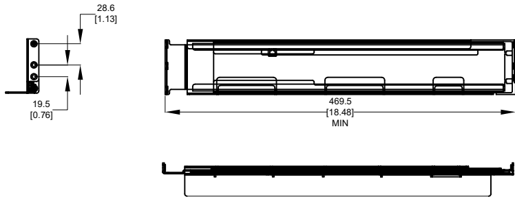
RAIL KIT LEFT SIDE
