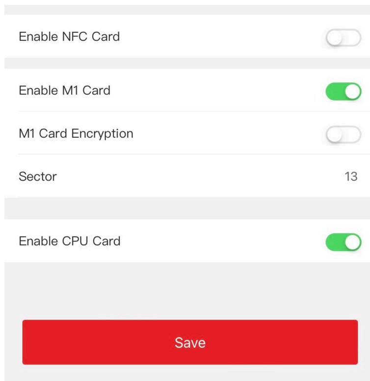
Figure 8-8 Card Security
