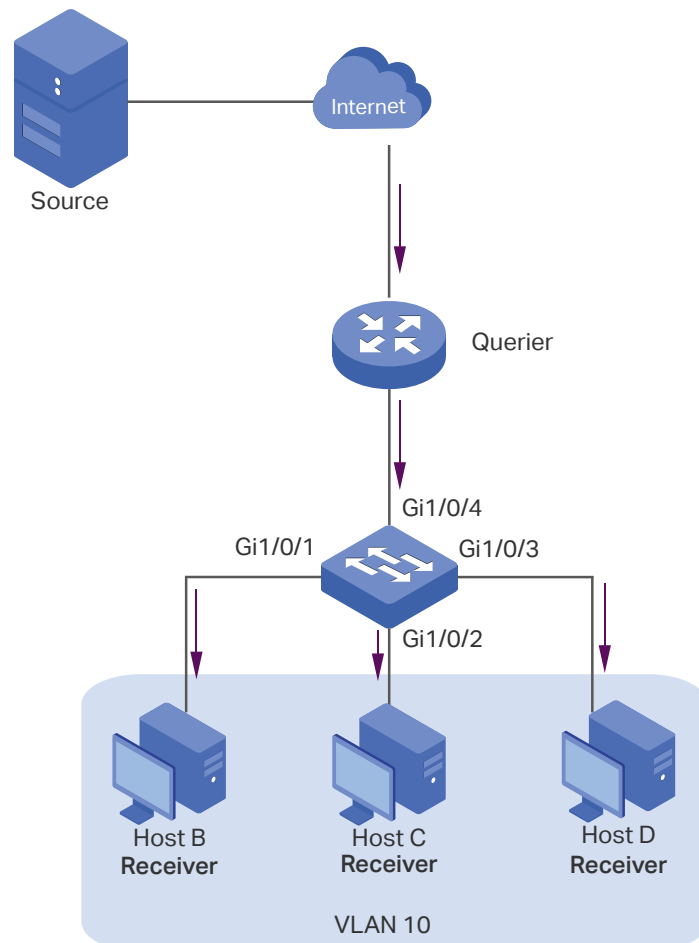
Figure 10-1 Network Topology for Basic IGMP Snooping
