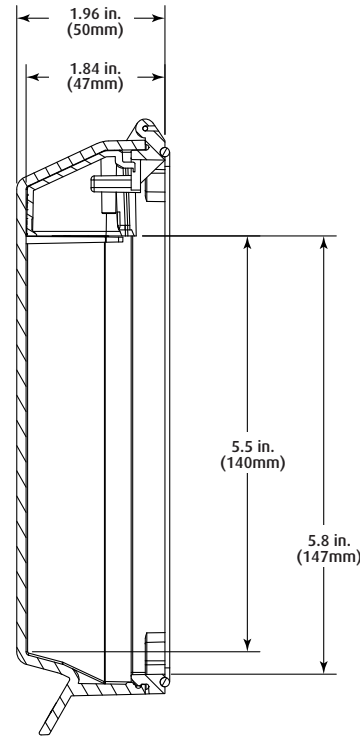
SECTION B-B
