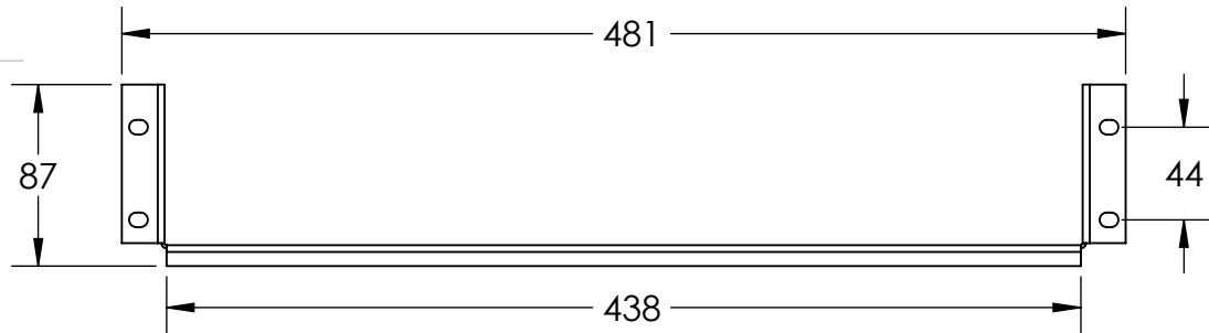
Vista frontal
