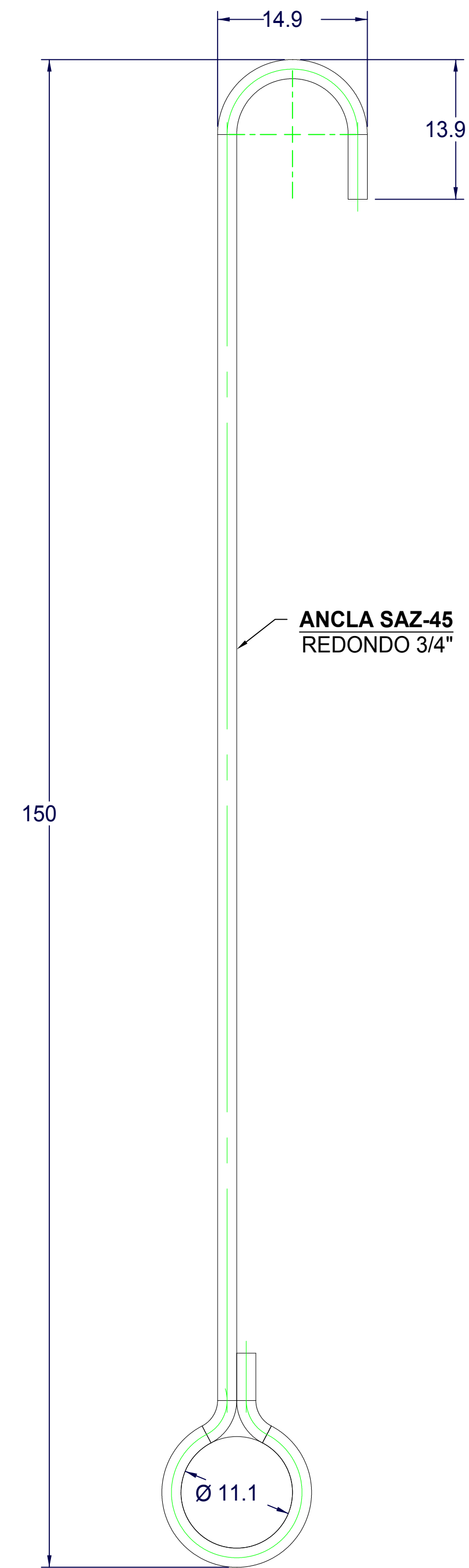
ANCLA SAZ-45 RDO 3/4"
