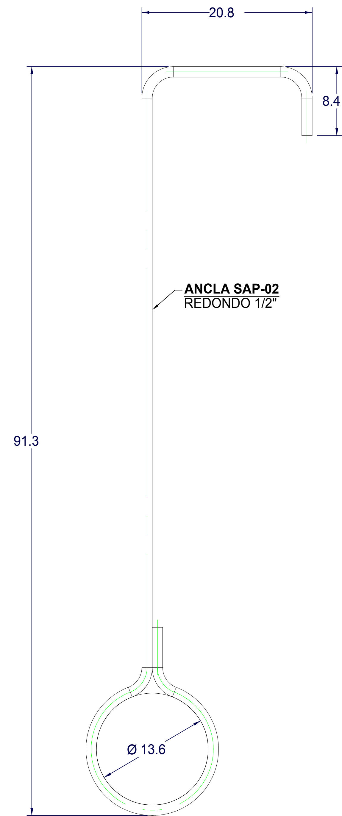
ANCLA SAP-02 RDO 1/2"
