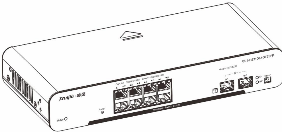
Figure 1-8 Appearance of RG-NBS3100-8GT2SFP
