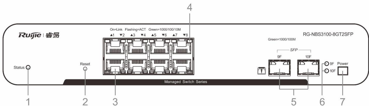
Figure 1-9 Front Panel of RG-NBS3100-8GT2SFP
