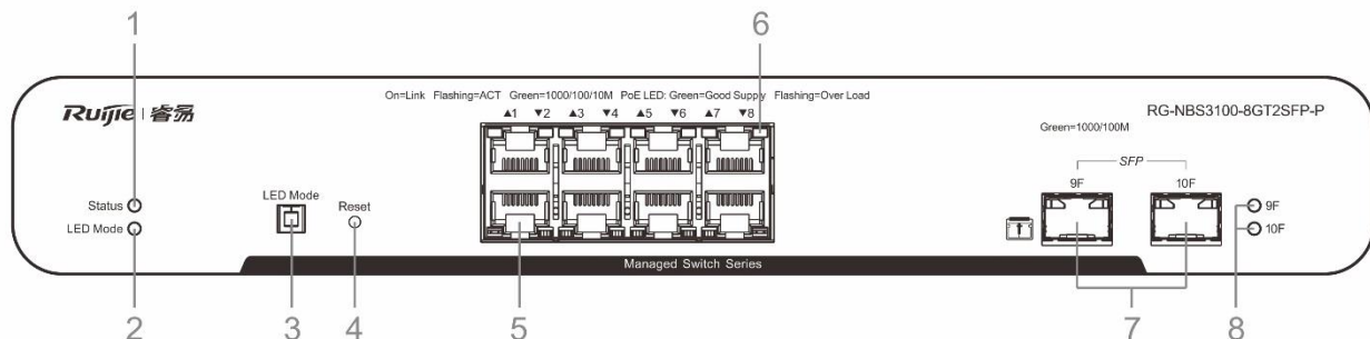
Figure 1-12 Front Panel of RG-NBS3100-8GT2SP-P
