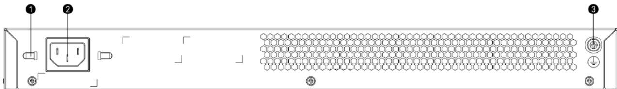
Figure 1-3 Back Panel of RG-NBS3100-24GT4SFP
