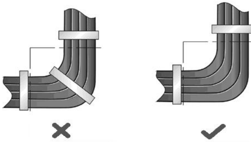
Figure 6-5 Binding Cables (3)
