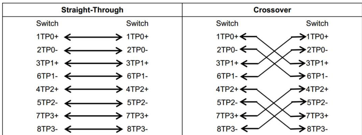
Figure 6-1 1000BASE-T Connection
