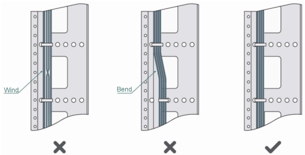
Figure 6-3 Binding Cables (1)
