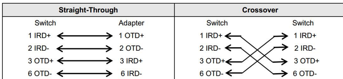
Figure 6-2 100BASE-TX/10BASE-T Connection
