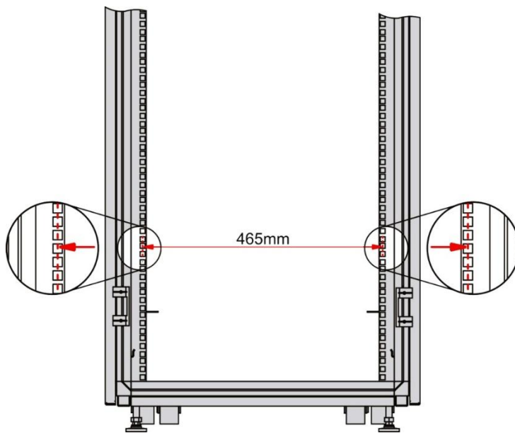
Figure 2-2 Standard 19-inch Cabinet
