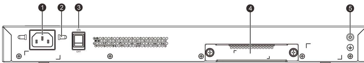
Figure 1-4 Back Panel of RG-EG1510XS
