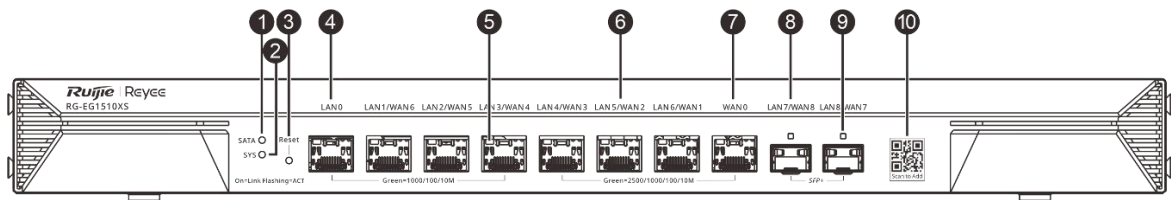
Figure 1-3 Front Panel of RG-EG1510XS
