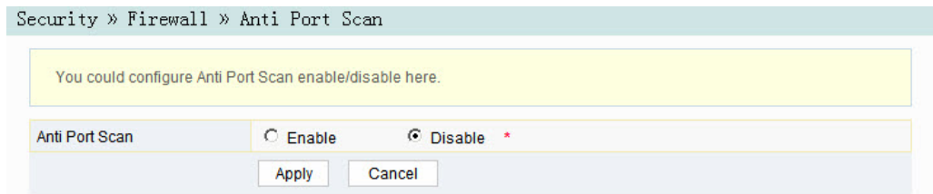
Figure 3-28 Anti-port Scan
