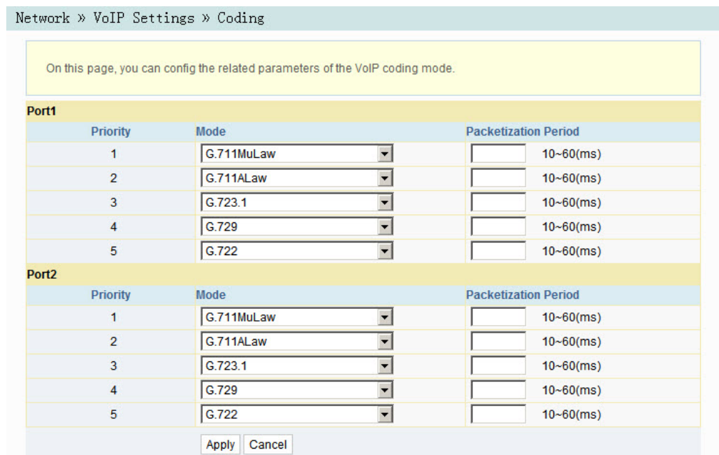
Figure 3-22 Coding
