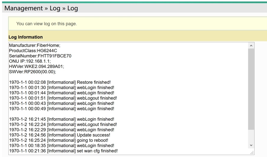
Figure 3-48 Log
