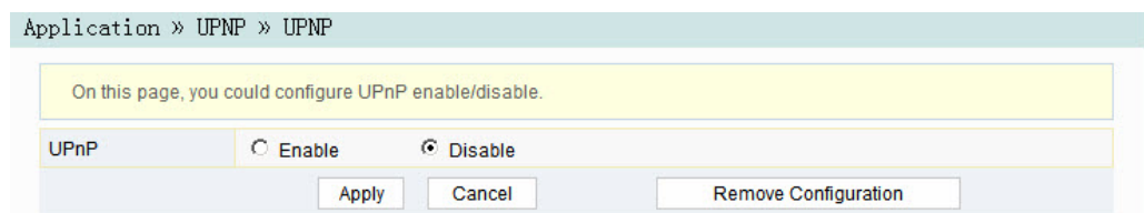
Figure 3-37 UPnP
