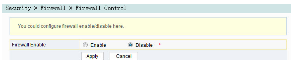
Figure 3-23 Firewall Enabling
