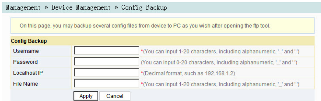
Figure 3-44 Configuration Backup
