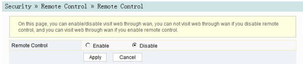
Figure 3-31 Remote Control
