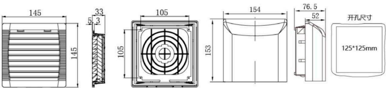
outline dimensional diagram
