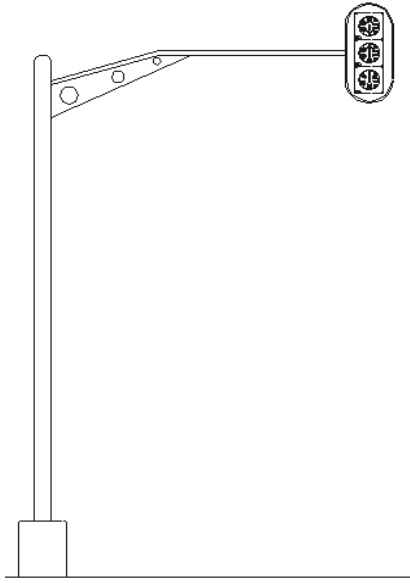
Vertical installation
