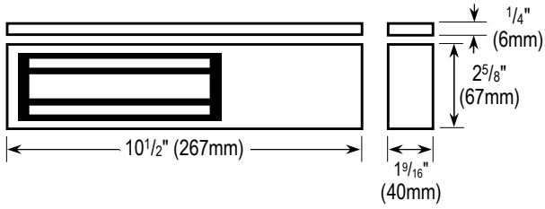
Electroimán
