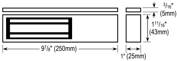
Electroimán
