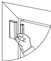
Figure 8: Battery/enrollment tab
