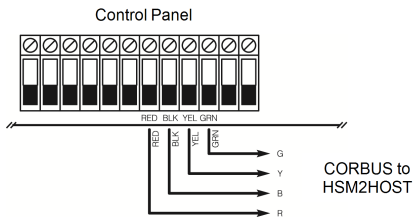
Figure: 1 Wiring Diagram
