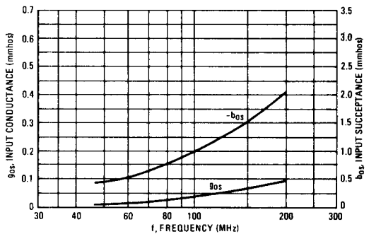
FIGURE 4 – OUTPUT ADMITTANCE
