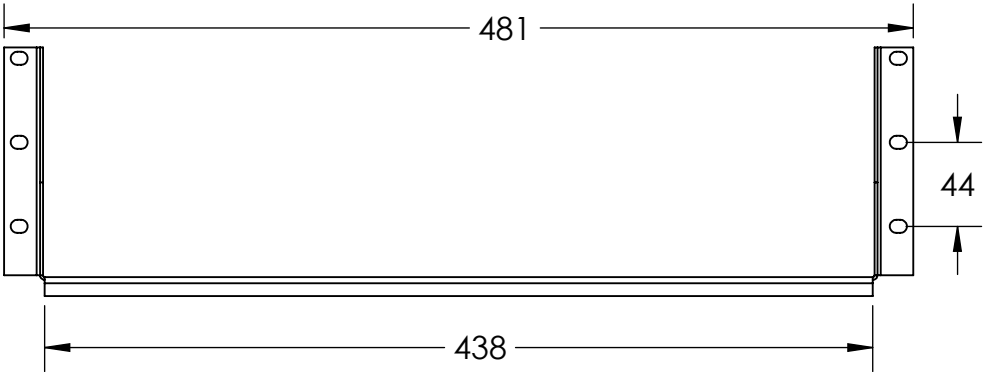
Vista frontal
