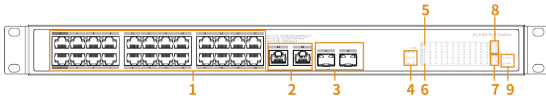
Figura 2-3 Panel frontal
