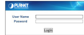
Figure 4-2: Login Screen
