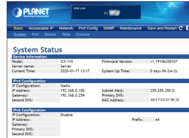
Figure 4-3: Web Main Screen of Serial Device Server
