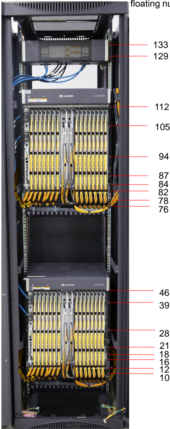
Cabinet configured with 2 EA5800-X15 subracks
