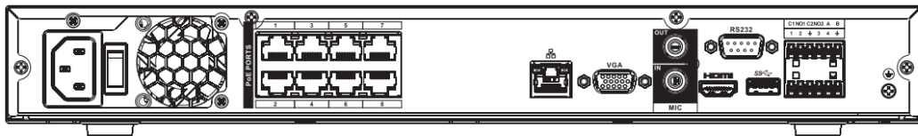
Figura 2-35 Panel trasero
