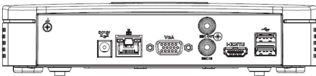
Figura 2-25 Panel trasero
