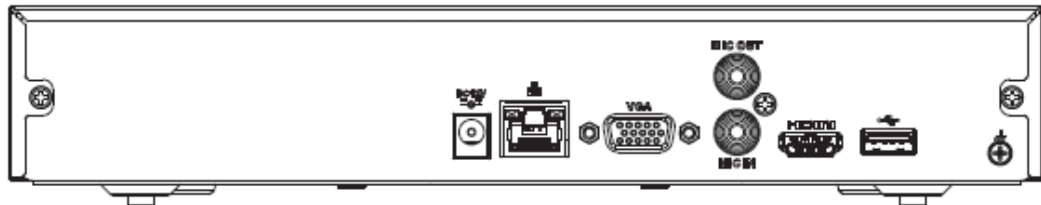
Figura 2-28 Panel trasero
