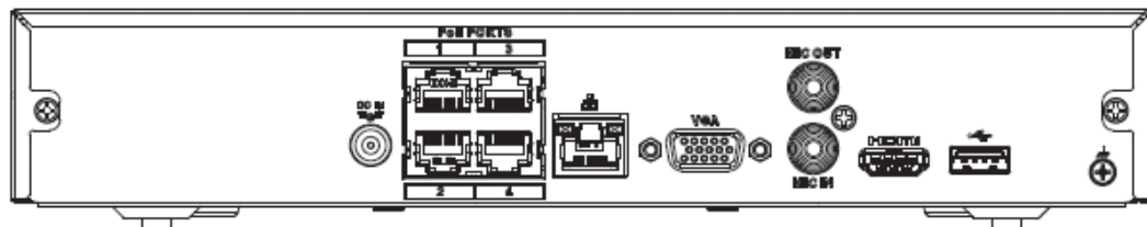
Figura 2-29 Panel trasero
