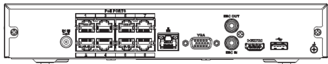
Figura 2-30 Panel trasero
