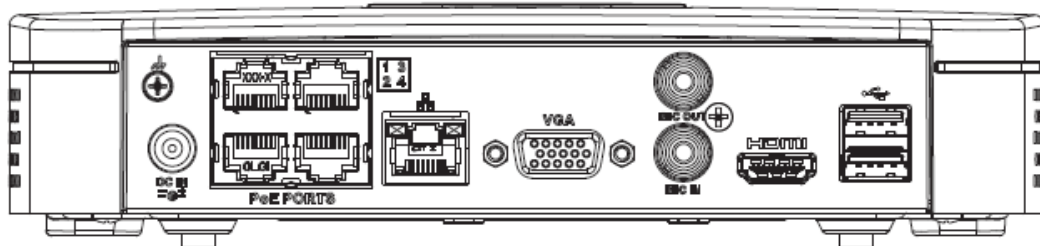
Figura 2-26 Panel trasero
