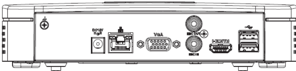
Figura 2-44 Panel trasero
