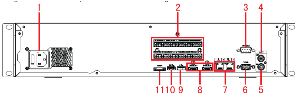
Figura 2-75 Panel trasero
