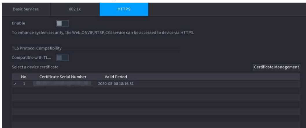
Figura 5-240 HTTPS
