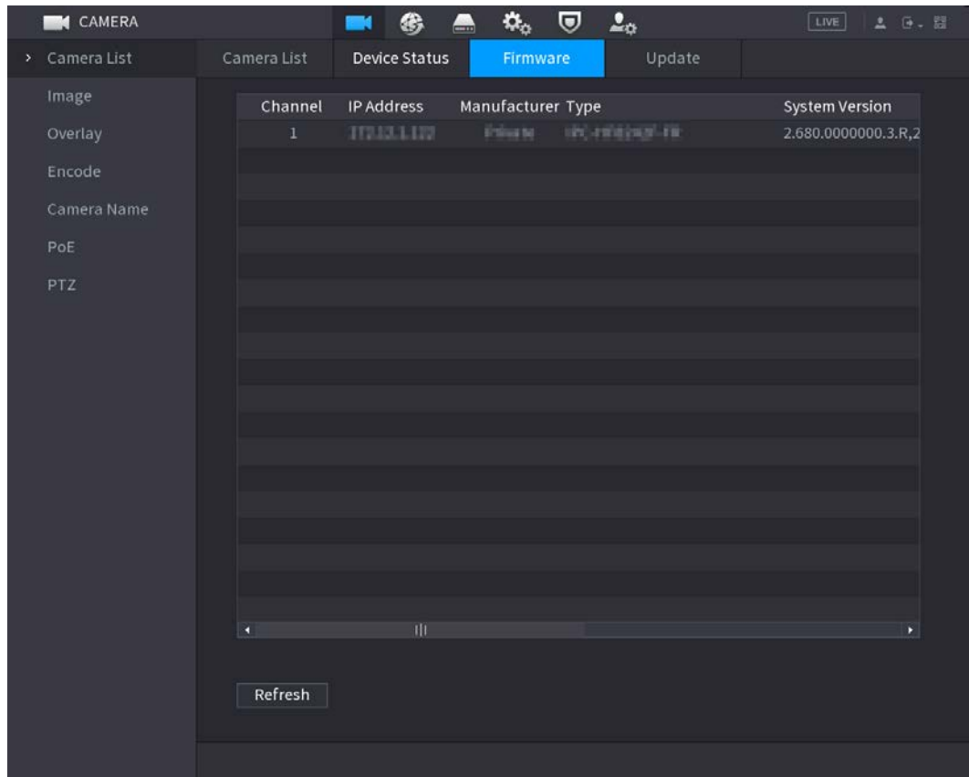
Figura 5-64 Firmware
