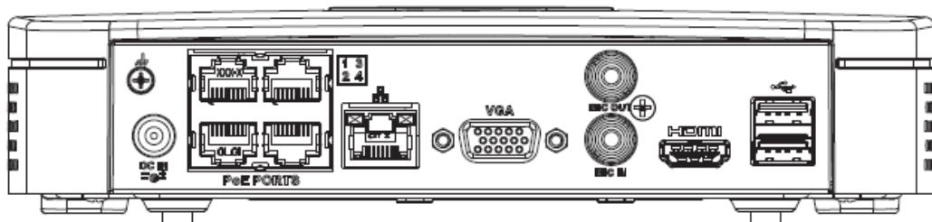
Figura 2-45 Panel trasero
