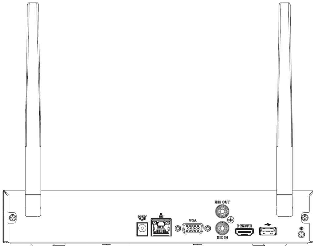
Figura 2-79 Panel trasero
