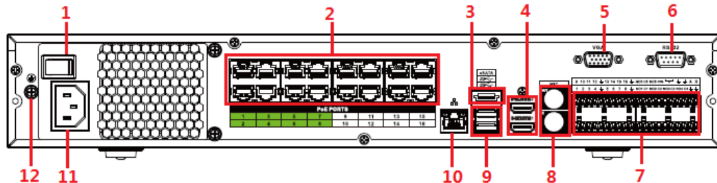
Figura 2-70 Panel trasero
