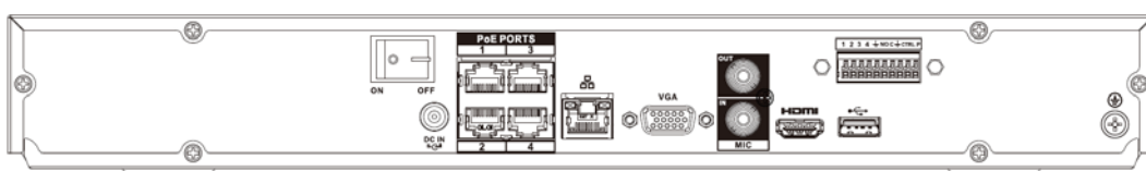
Figura 2-48 Panel trasero
