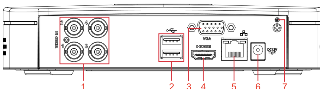
Figure 3-20 Panel trasero
