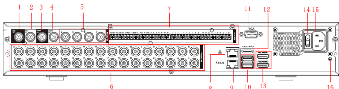
Figure 3-18 Panel trasero
