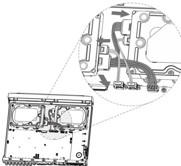
Figure 2-5 Conectar cables
