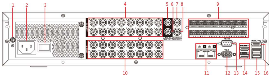
Figure 3-16 Panel trasero
