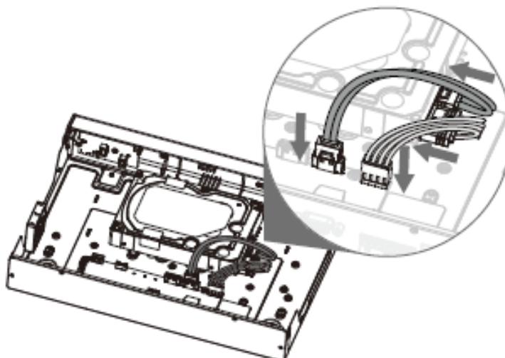
Figure 2-27 Conectar cables
