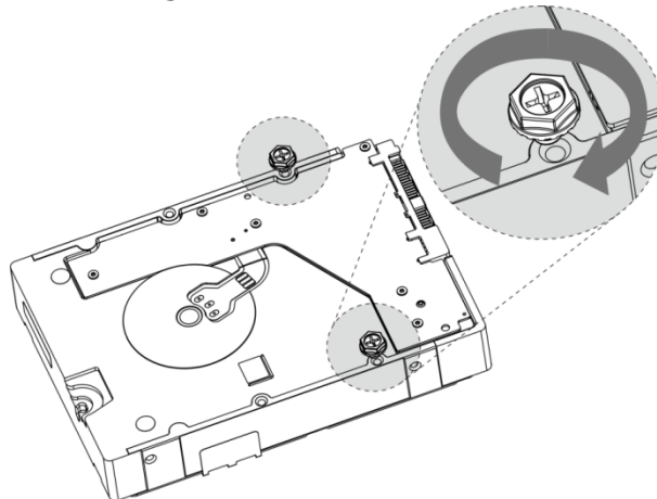
Figure 2-2 poner tornillos
