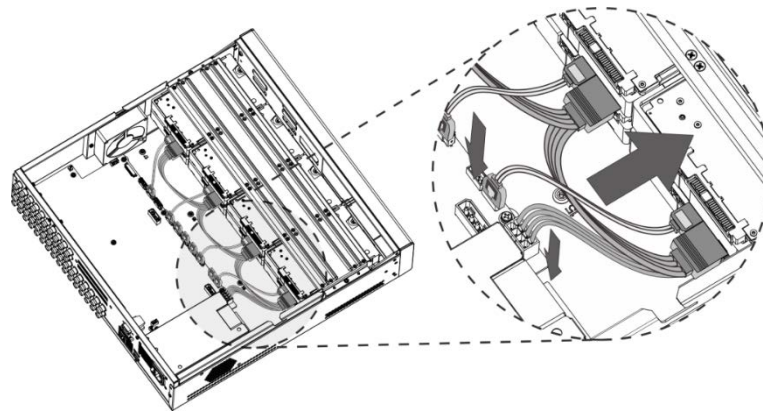
Figure 2-14 Conectar cables
