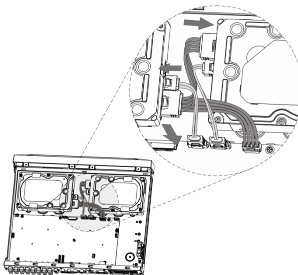
Figure 2-5 Conectar cables
