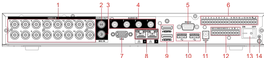
Figure 3-15 Panel trasero
