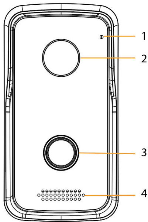
Figura 1-6 Panel frontal
