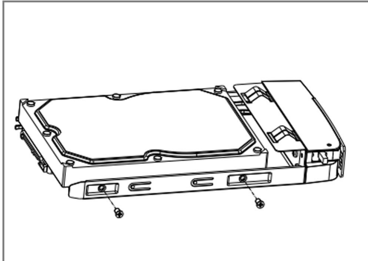
Figure 1-8 Fix HDD
