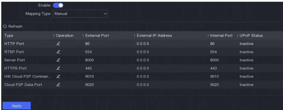
Figure 7-4 NAT
