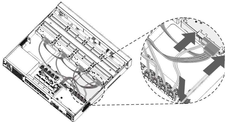
Figure 2-22 Conectar cables
