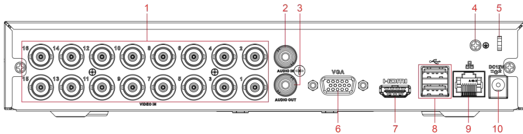
Figure 3-19 Panel trasero
