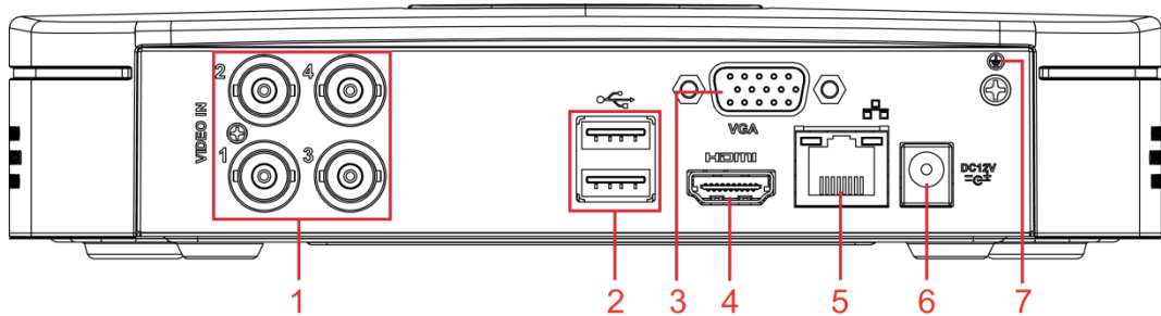
Figure 3-20 Panel trasero
