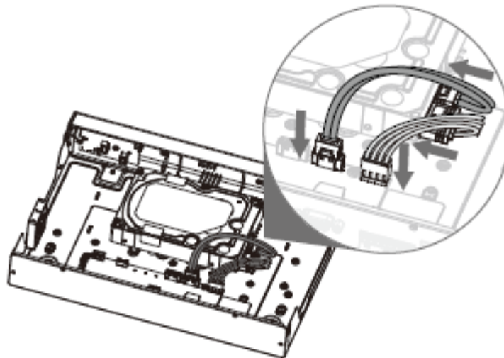
Figure 2-27 Conectar cables
