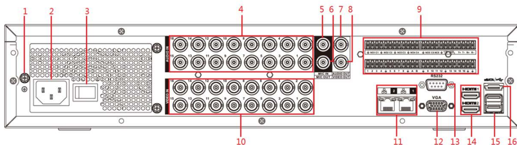
Figure 3-16 Panel trasero
