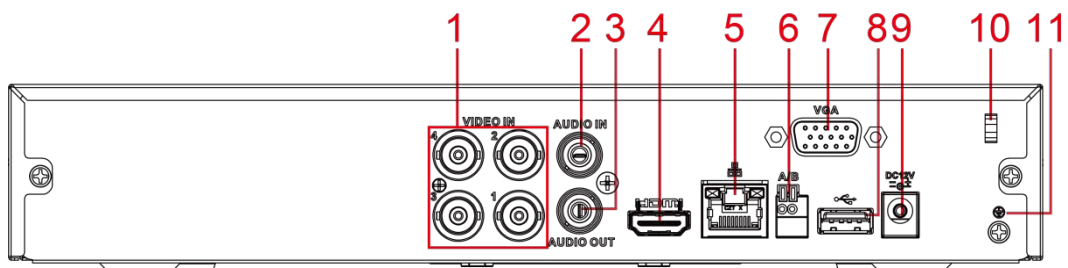
Figure 3-13 Panel trasero
