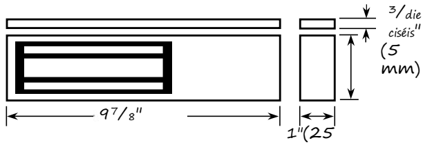
Electroimán
