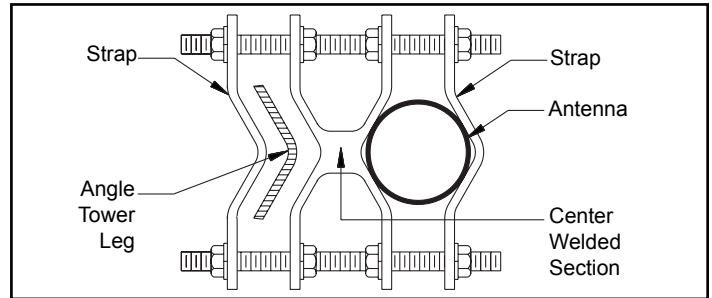
Figure 2. Mounting on Angle Tower Legs.
