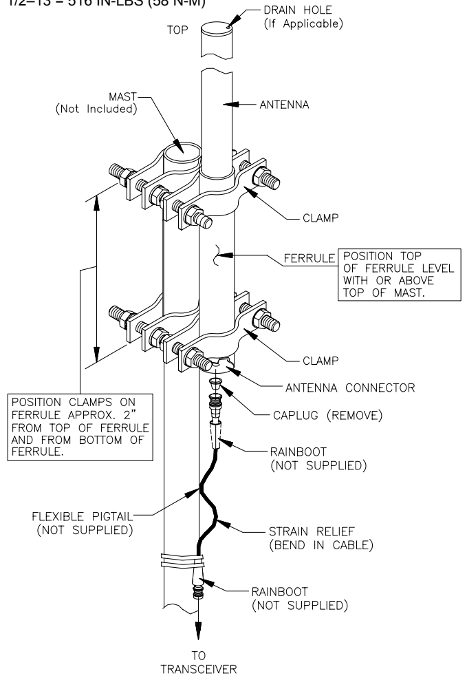
Figure 4. Upright Mounting of Antenna.
