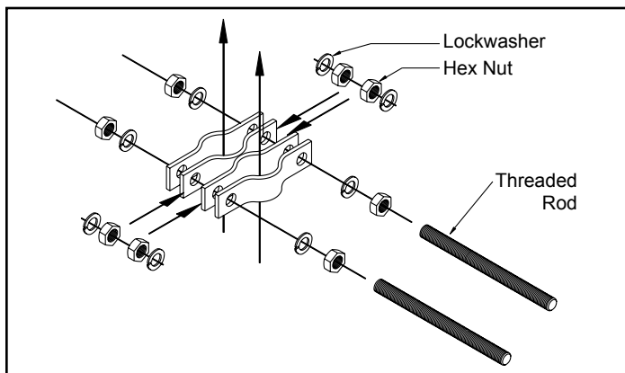
Figure 3. Mounting Clamp Hardware.
