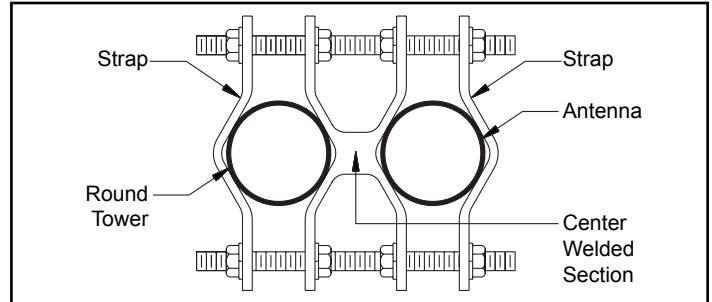
Figure 1. Mounting on Round Tower Legs.
