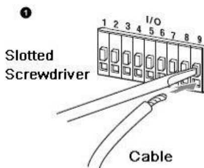
Figure 9-4 Instalar cable
