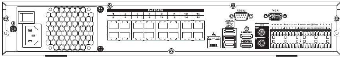
Figura 2-62 Panel trasero
