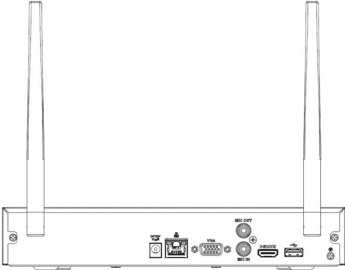
Figura 2-117 Panel trasero
