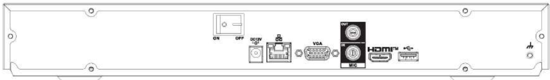
Figura 2-46 Panel trasero
