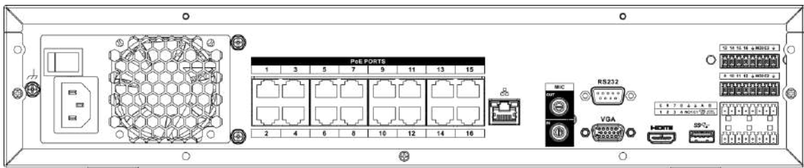
Figura 2-77 Panel trasero
