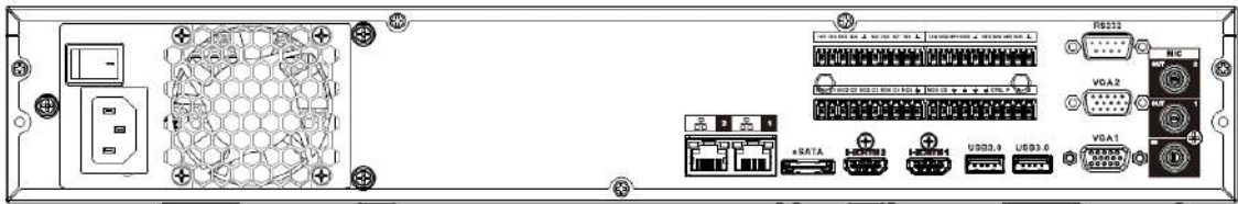
Figura 2-118 Panel trasero
