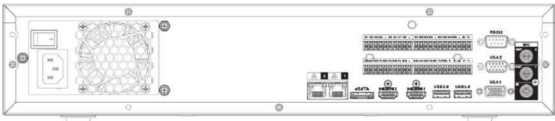
Figura 2-119 Panel trasero
