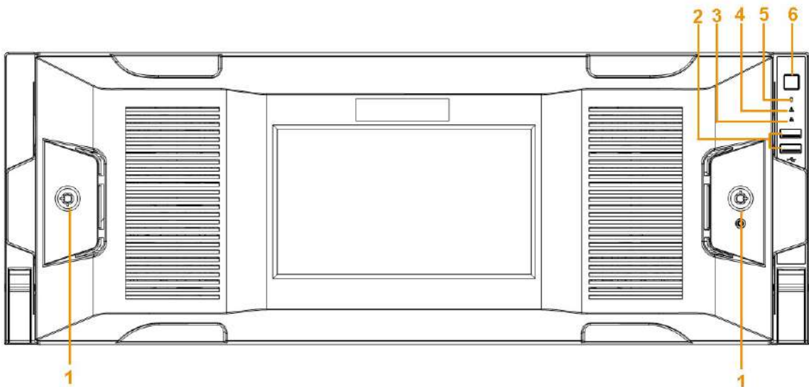
Figura 2-35 Panel frontal
