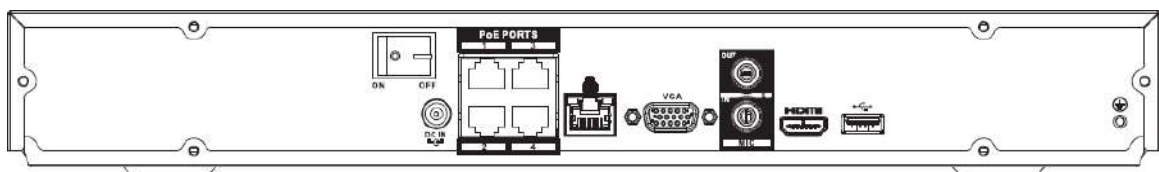
Figura 2-87 Panel trasero
