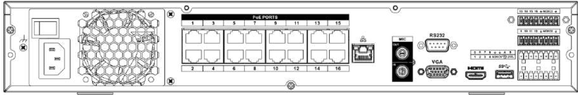
Figura 2-74 Panel trasero
