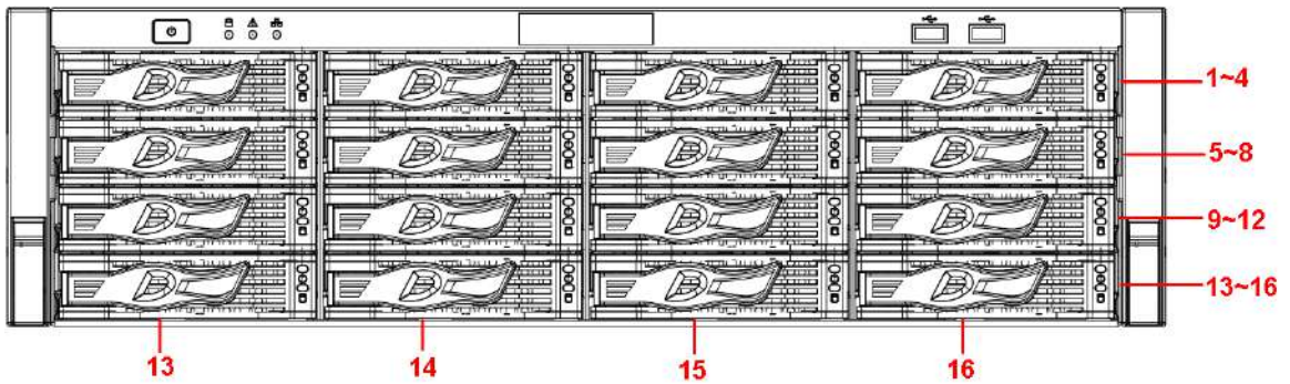
Figura 2-34 Panel frontal
