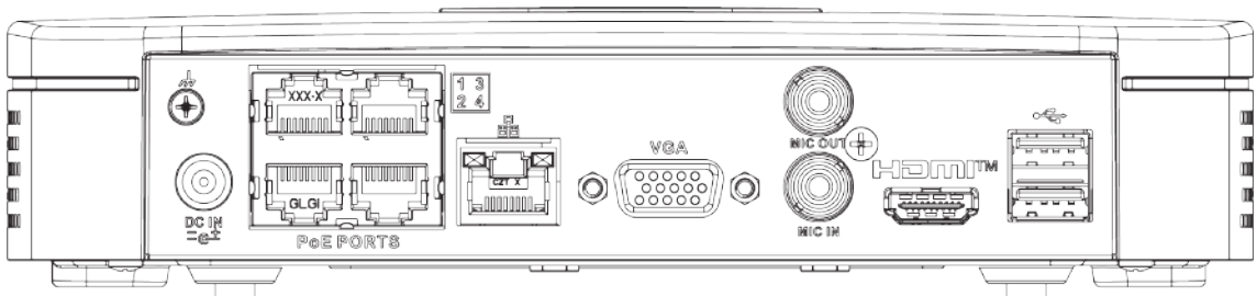
Figura 2-38 Panel trasero
