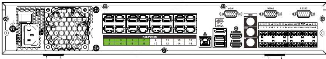
Figura 2-64 Panel trasero
