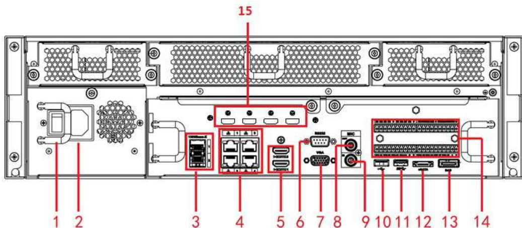
Figura 2-112 Panel trasero
