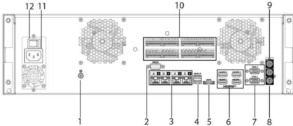
Figura 2-114 Panel trasero
