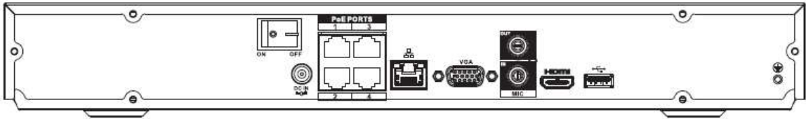
Figura 2-44 Panel trasero
