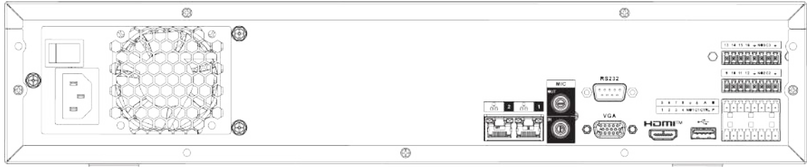
Figura 2-76 Panel trasero
