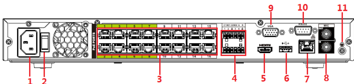
Figura 2-103 Panel trasero
