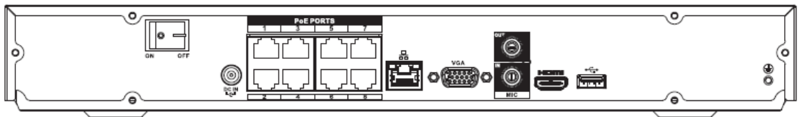
Figura 2-45 Panel trasero
