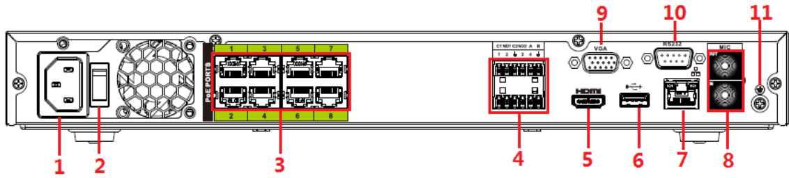
Figura 2-104 Panel trasero
