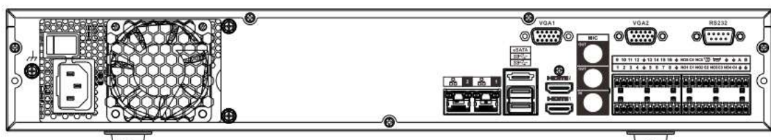
Figura 2-61 Panel trasero
