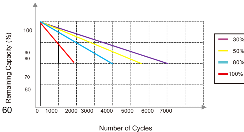
Different DOD Discharge Cycle Life Curve @ 1C
