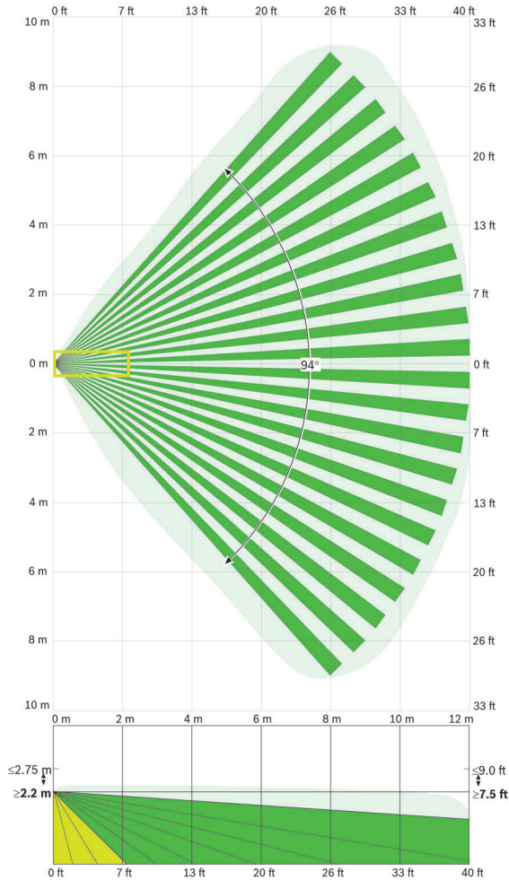
Cobertura de 12 x 12 m (40 x 40 pies)
