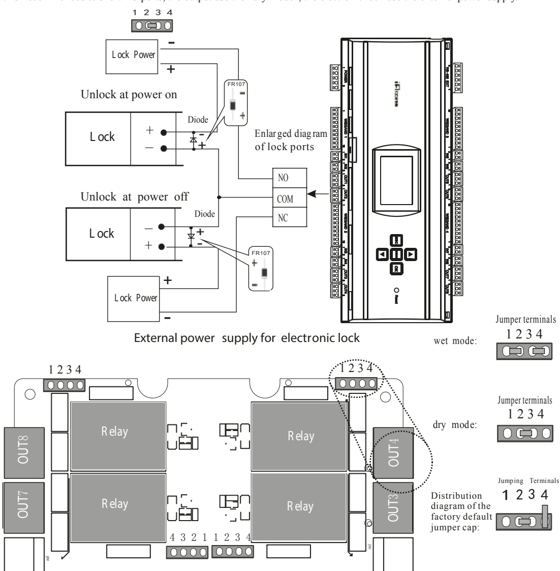
Relay output ports and jumper terminals setting (The second layer of PCB)
