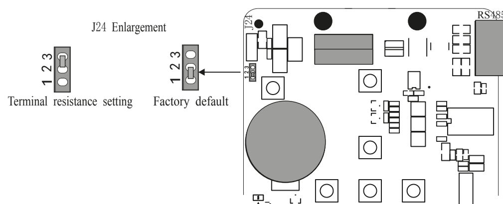
Terminal resistance setting diagram (The first layer of PCB)
