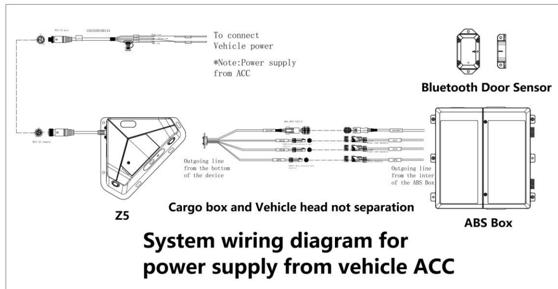
System connection diagram ( Powered from ACC power )
