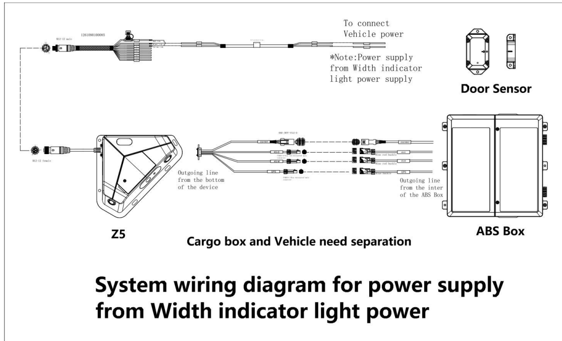
System connection diagram ( Powered from the width indicator light power )
