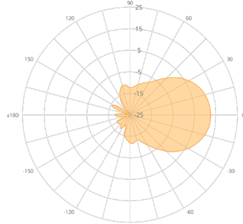
N5-X12 (12 dBi)
