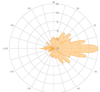
N5-X25 (25 dBi)
