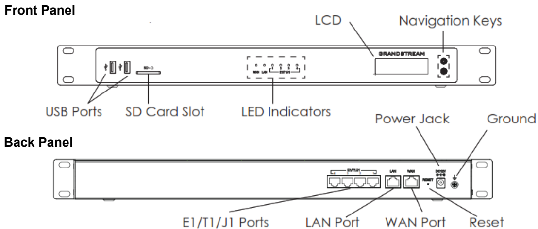
Figure: Diagram of GXW4504 Back and Front Panel
