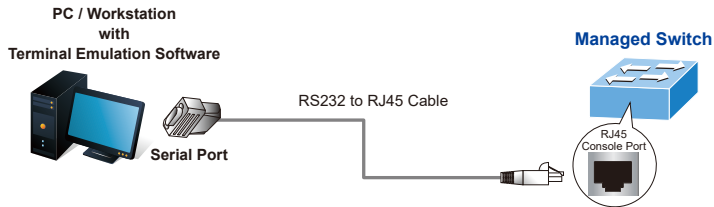
Figure 5-1: Managed Switch Console Connectivity
