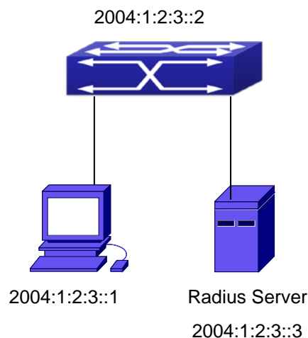
Fig 3-17 IPv6 Radius
