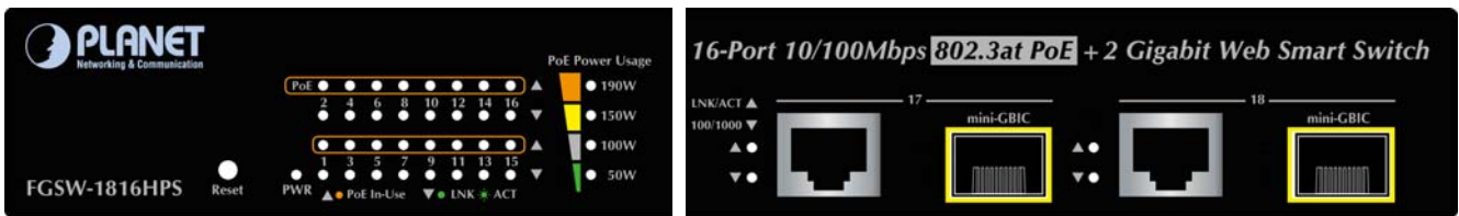
Figure 2-2-B FGSW-1816HPS LED panel
