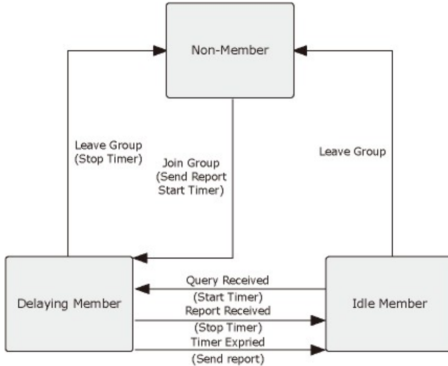
Figure 4-12-4 IGMP State Transitions
