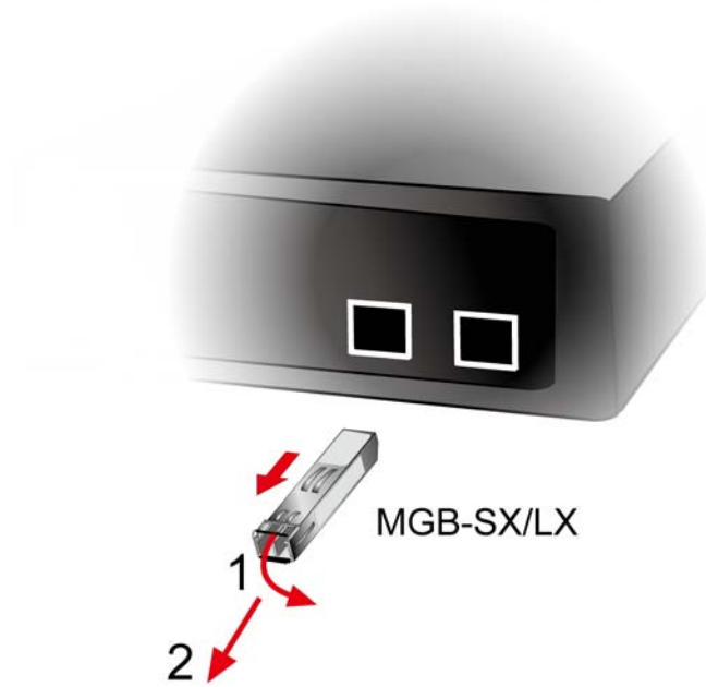
Figure 2-8 How to Pull Out the SFP Transceiver
