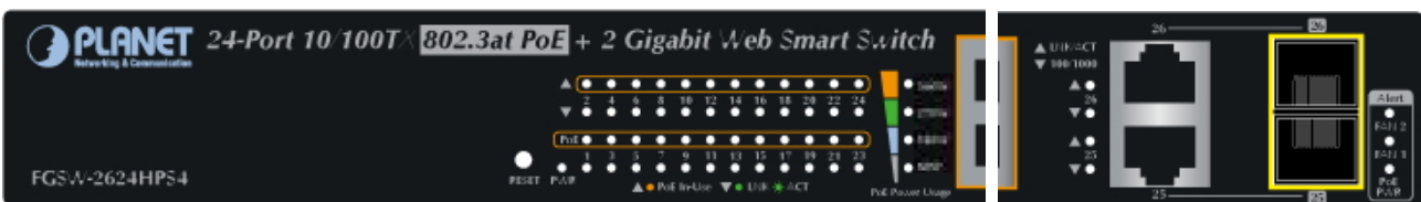
Figure 2-2-D FGSW-2624HPS4 LED panel
