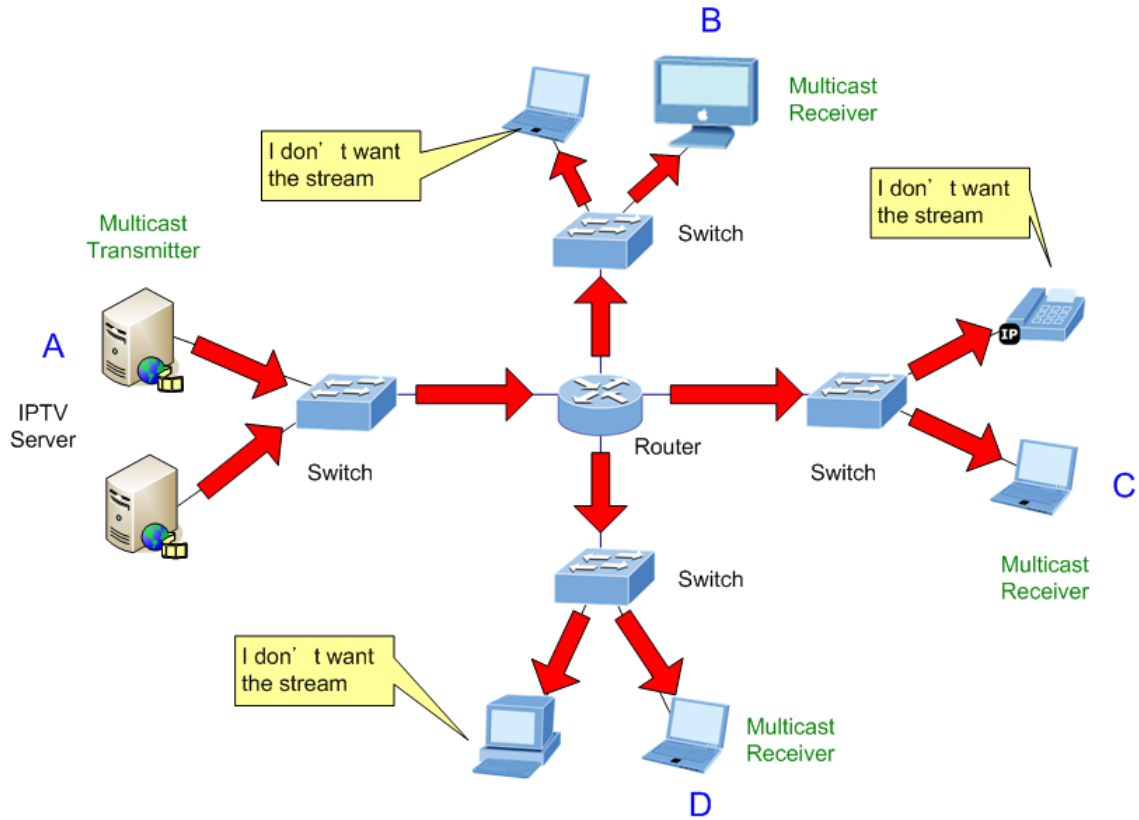
Figure 4-12-2 Multicast Flooding
