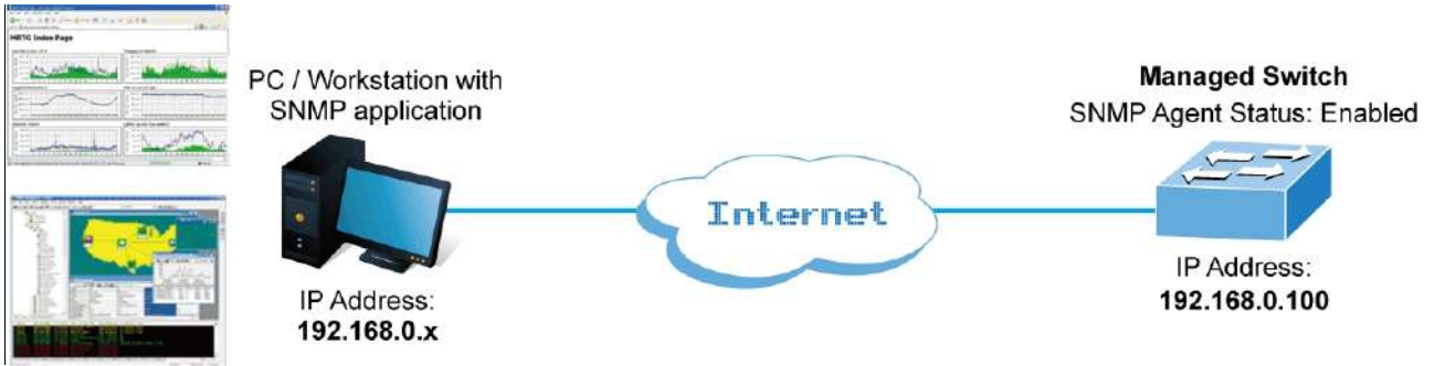
Figure 3-1-5: SNMP Management
