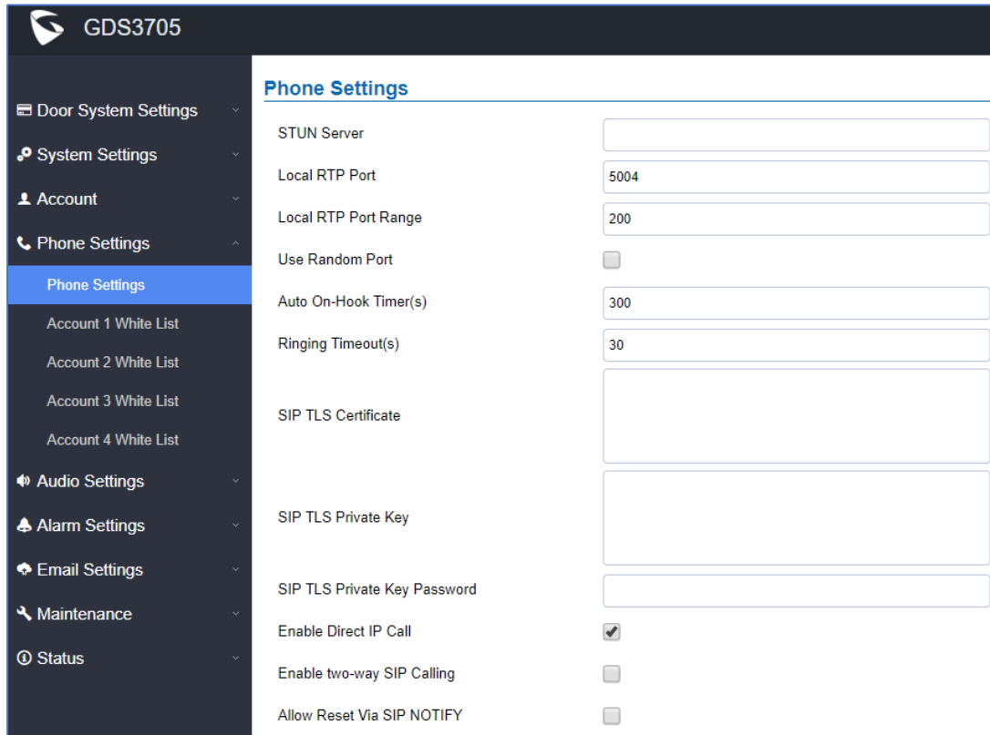
Figure 64: Phone Settings Page
