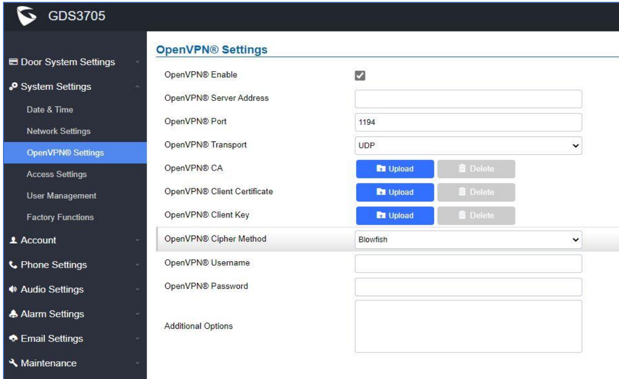
Figure 57: OpenVPN Settings page
