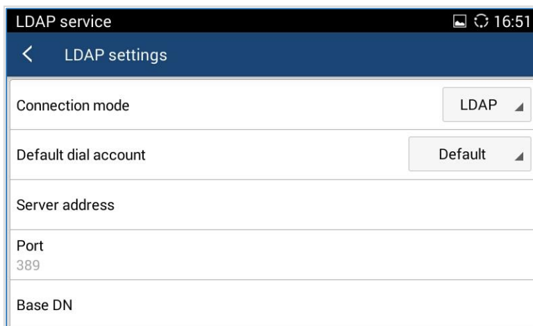
Figure 77: GAC2500 LDAP Settings
