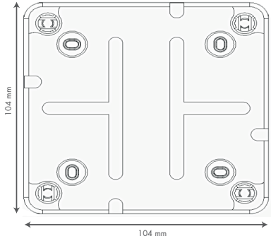
CAJA ESTANCA IP55 100x100x50 mm
