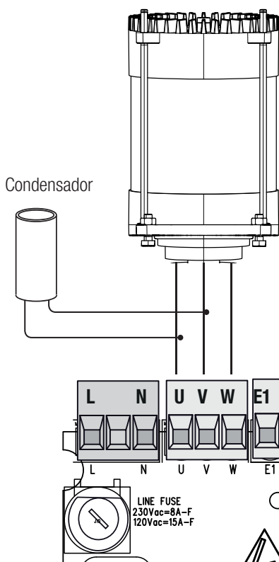
Motorreductor 120/230V (AC)
