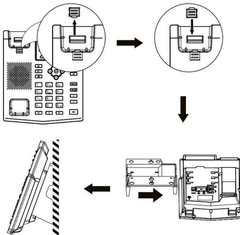
Picture 2 - Wall-mounted installation
